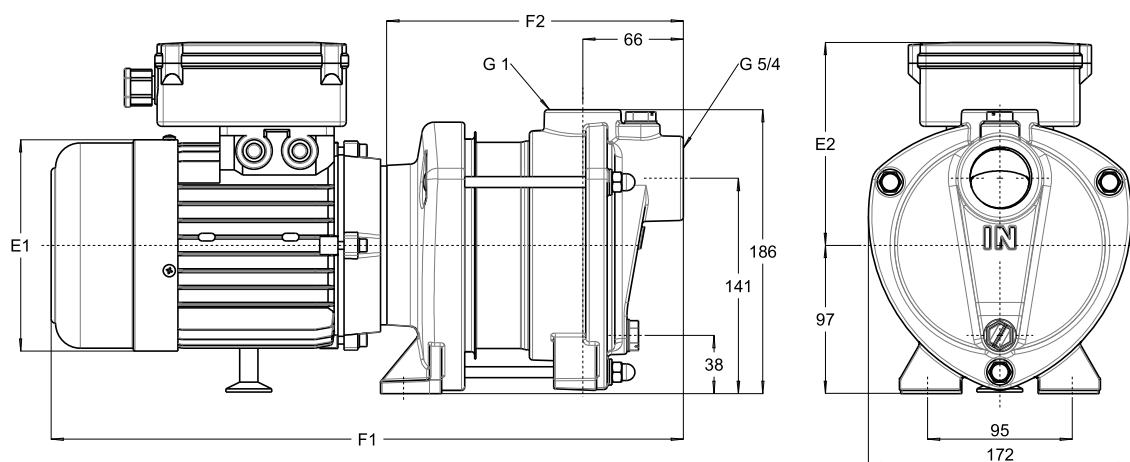
Figure 3: Pump dimensions
